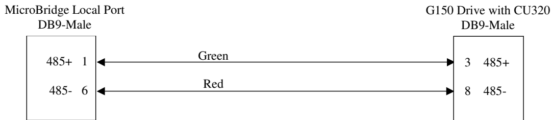
Figure 2 - G150/W150(CP) with CU320 Profibus Cable
