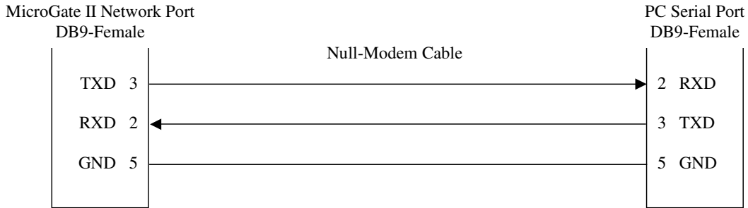
Figure 3 - Configuration Cable
