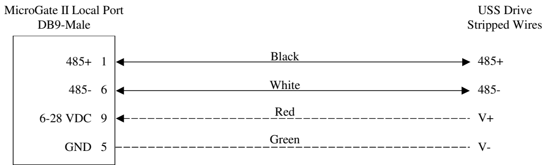
Figure 2 - USS Drive Cable
